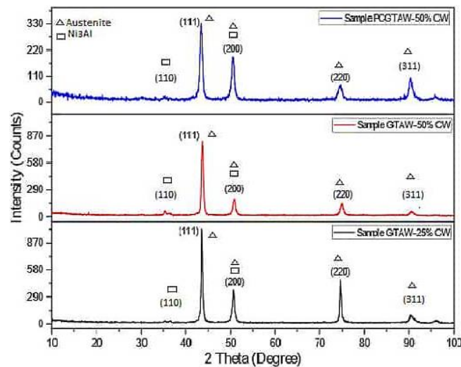
Fig. 8. XRD analysis of Nimonic 80A weldments of GTAW and PCGTAW samples
